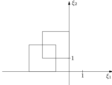
Figure 2. In order to represent the 2-clause y_1^1 \vee y_2^{-1} , all visibility rays in the orthant \xi_1 \leq 0, \xi_2 \geq 0 have to be blocked. This can be achieved by placing two unit squares centered at (-2, 1)^T and (-1, 2)^T .
