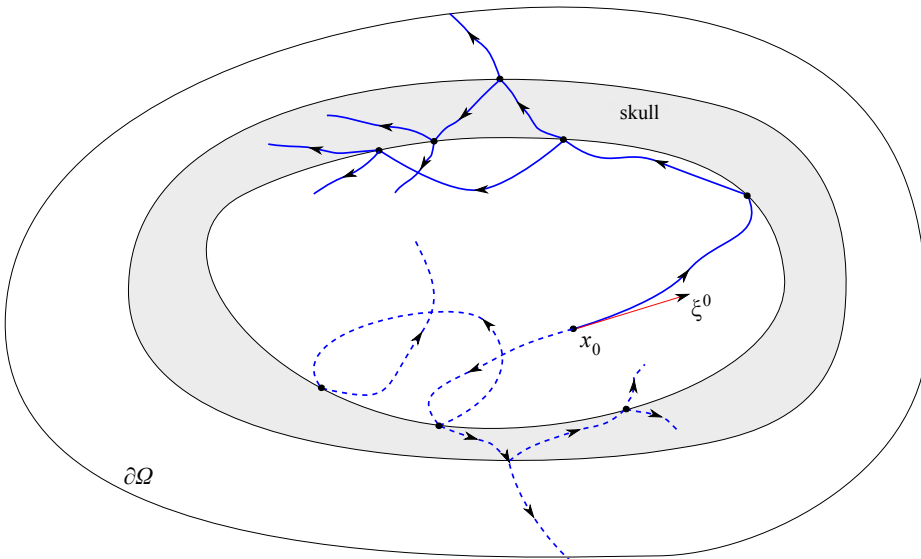
Figure 2. Propagation of singularities for the transmission problem in the skull example. The shaded region represents the skull, and the speed there is higher than in the nonshaded part. The dotted curves represent the propagation of the same singularity but moving with a negative wave speed.
