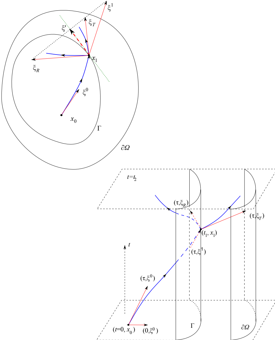
Figure 3. Reflected and the transmitted rays in x -space (top) and in (t, x) -space (bottom).
